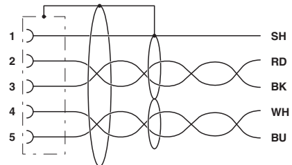
Circuit diagram
